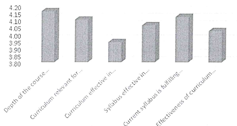
Employers Feedback (Average)
